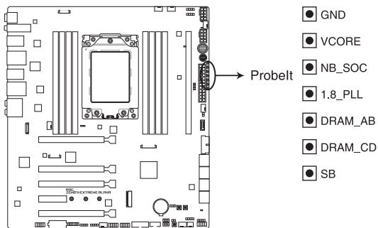
ROG ZENITH EXTREME ALPHA Probelts
