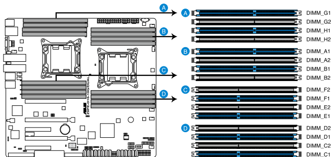
Z9PE-D16-10G Series 240-pin DDR3 DIMM sockets
