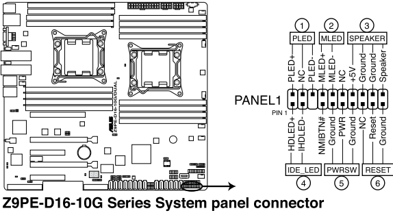
Z9PE-D16-10G Series System panel connector
