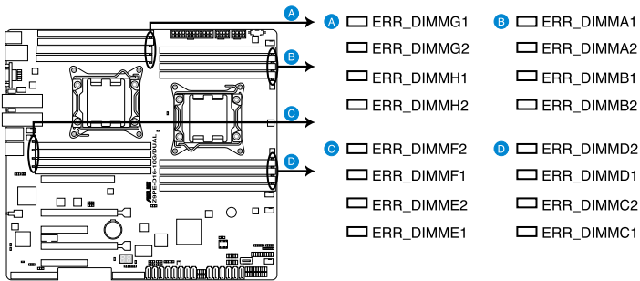
Z9PE-D16-10G Series ERR DIMM LED
