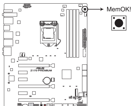
Z170-PREMIUM MemOK! button
