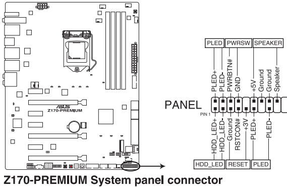
Z170-PREMIUM System panel connector
