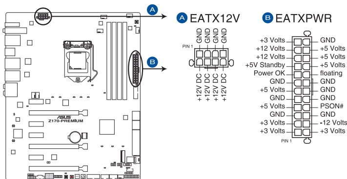
Z170-PREMIUM ATX power connectors
