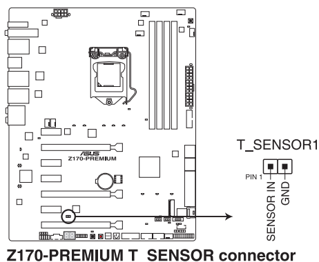
Z170-PREMIUM T_SENSOR1 connector
