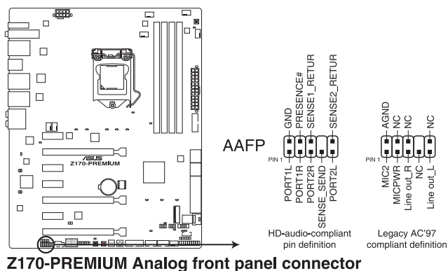
Z170-PREMIUM Analog front panel connector
