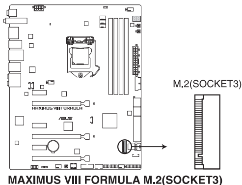
MAXIMUS VIII FORMULA M.2(SOCKET3)
