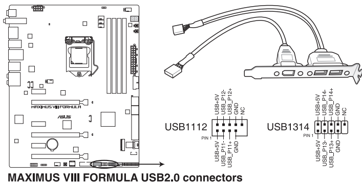
MAXIMUS VIII FORMULA USB2.0 connectors
