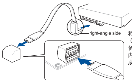
MAXIMUS VIII FORMULA Intel® SATA 6 Gb/s connectors
