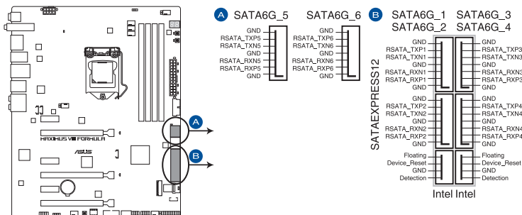
MAXIMUS VIII FORMULA Intel® SATA 6 Gb/s connectors
