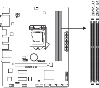
H110M-E D3 240-pin DDR3 DIMM sockets
