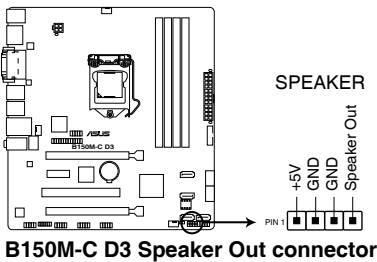
B150M-C D3 Speaker Out connector
