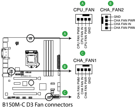
B150M-C D3 Fan connectors
