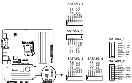
B150M-C D3 Intel® SATA 6 Gb/s connectors
