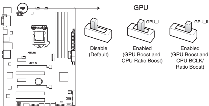
Z97-C GPU Boost switch
