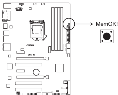
Z97-C MemOK! button
