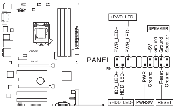
Z97-C System panel connector
