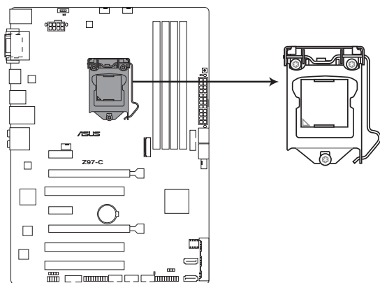
Z97-C CPU socket LGA1150
