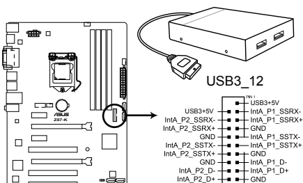
Z87-K USB3.0 front panel connector
