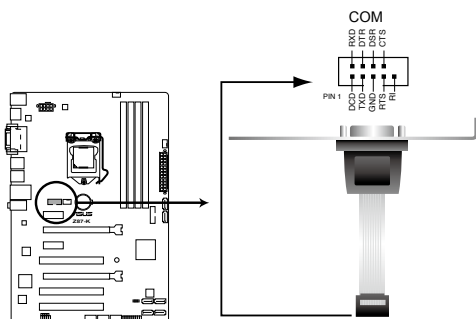
Z87-K Serial port (COM) connector
