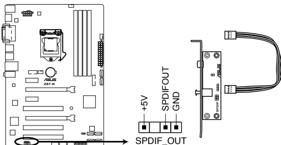
Z87-K Digital audio connector
