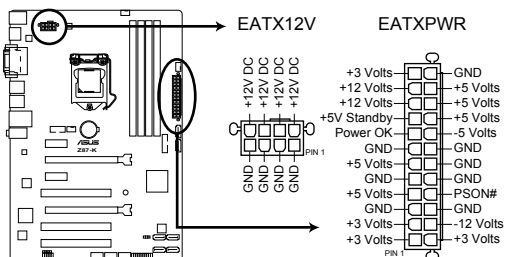
Z87-K ATX power connectors
