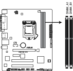
H81M-V3 240-pin DDR3 DIMM sockets
