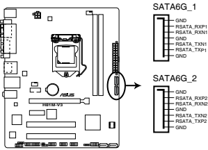
H81M-V3 SATA 6.0Gb/s connectors
