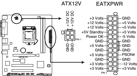
H81M-V3 ATX power connectors
